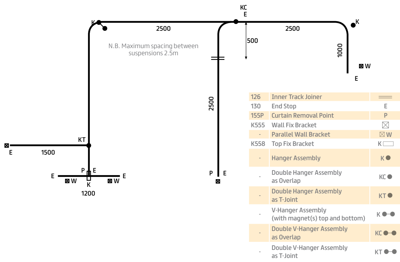
EXAMPLE ONLY of dimension drawing showing use of symbols based on isometric drawing
