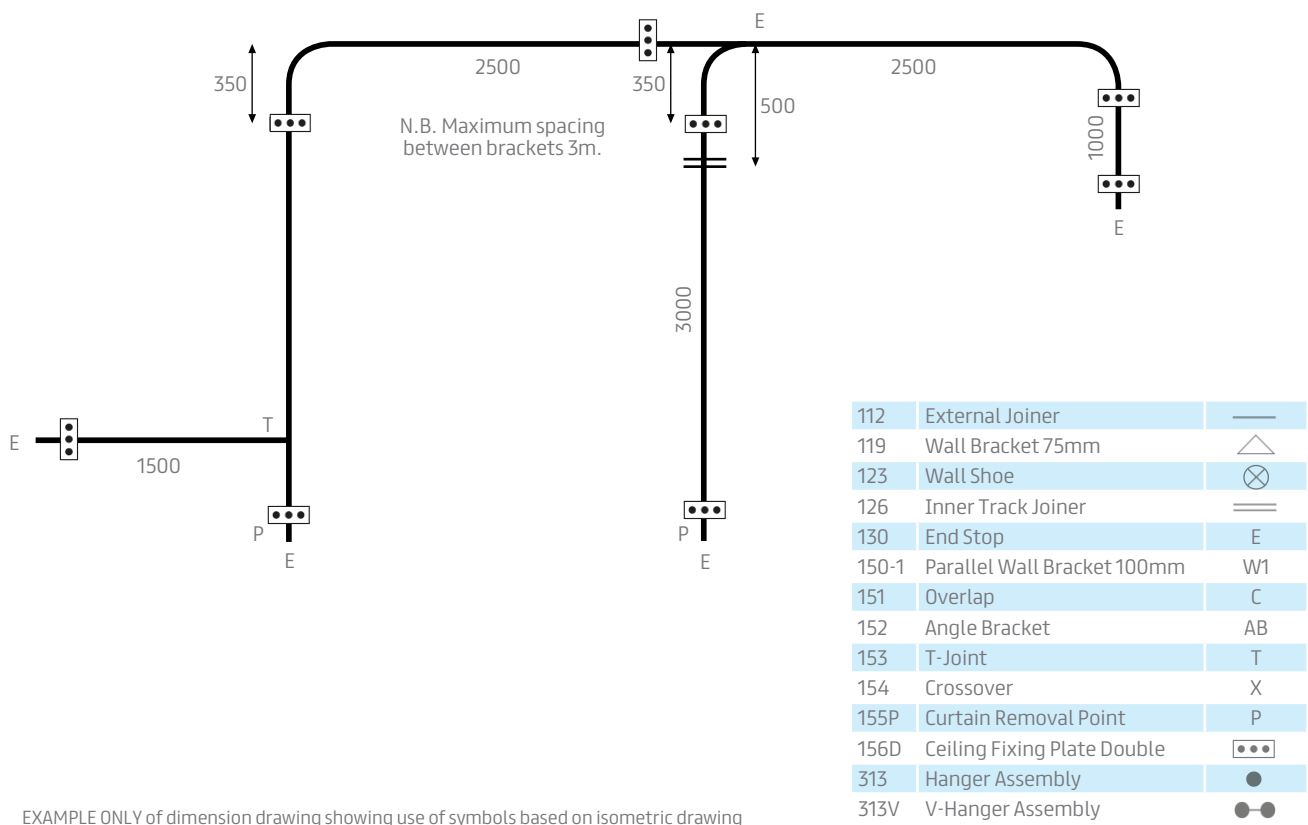
EXAMPLE ONLY of dimension drawing showing use of symbols based on isometric drawing
