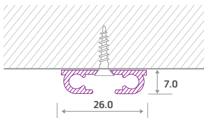
Direct top Fix
