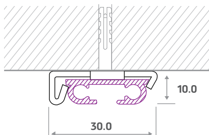
Bracket Top Fix
