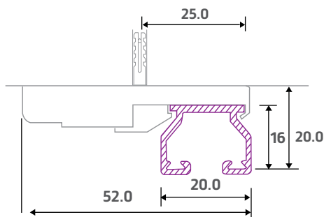
Top-fix
